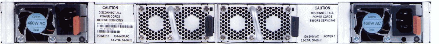
FortiSwitch 1048D – back
