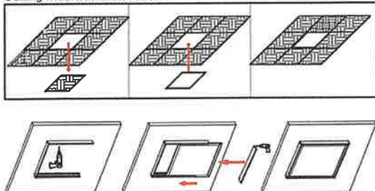
Ceiling Mounted Installation
