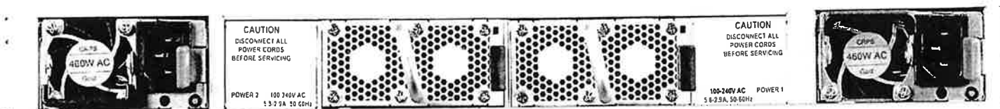
FortiSwitch 1024D — back
