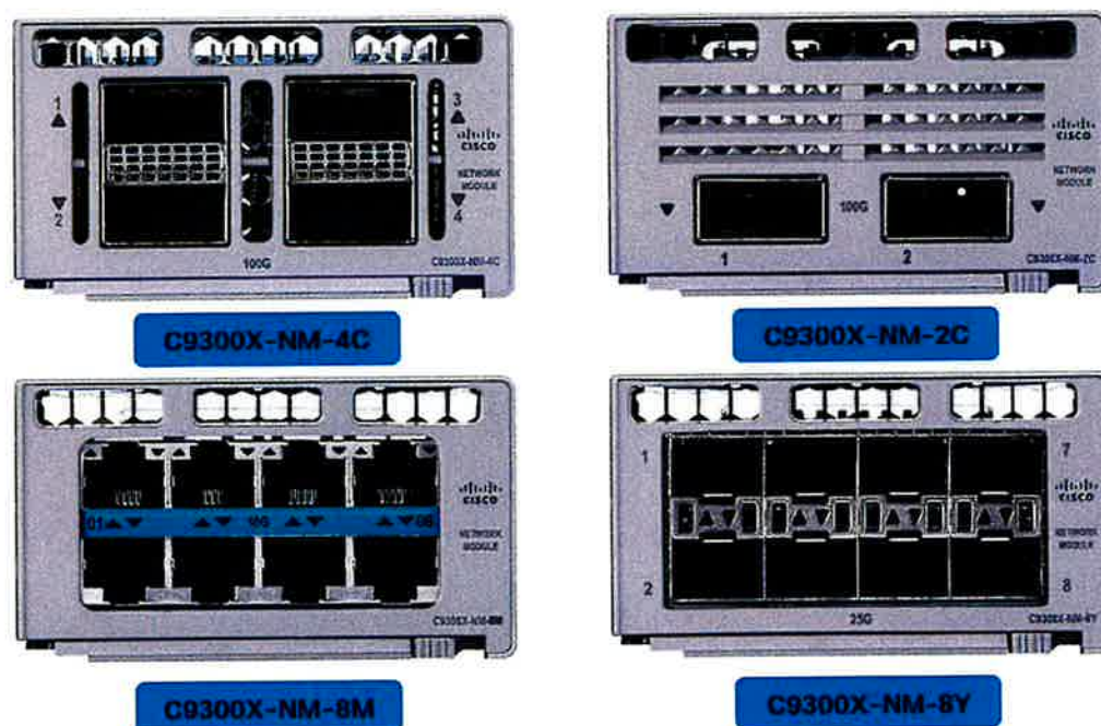
Figure 2. Cisco Catalyst 9300X network modules
