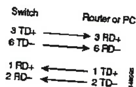
Figure 11: Two Twisted-Pair Crossover Cable Schematic
