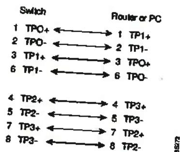
Figure 8: Four Twisted-Pair Straight-Through Cable Schematic
