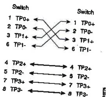
Figure 10: Two Twisted-Pair Straight-Through Cable Schematic
