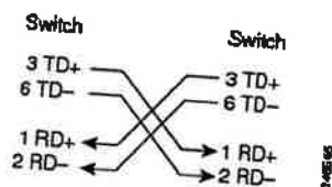
Figure 11: Two Twisted-Pair Crossover Cable Schematic
