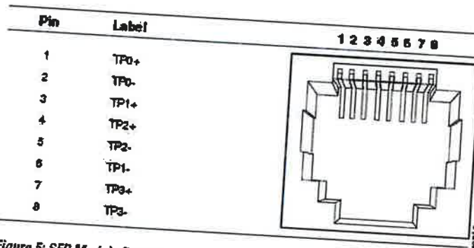
Figure 5: SFP Module Patch Cable
