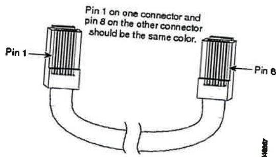
Figure 12: Identifying a Crossover Cable
