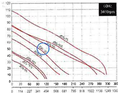
Performance Curve
