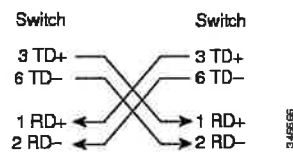
Figure 11: Two Twisted-Pair Crossover Cable Schematic
