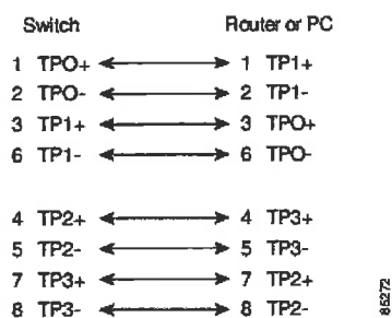
Figure 8: Four Twisted-Pair Straight-Through Cable Schematic
